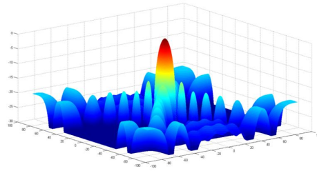
Fig (7): 3D intensity of the proposed 12×12-element TPA array
