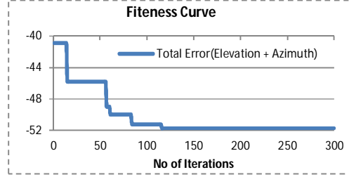
Fig (6): Variations in fitness value i.e. total PSLL values in both the planes ( \theta=0^0 and \theta=90^0 ) with number of iterations for the proposed 12×12-element TPA array
