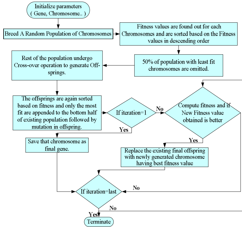
Fig (2): Flowchart of the proposed MBC-GA
